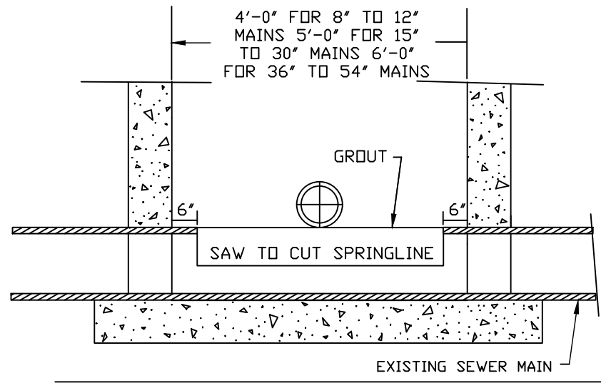
SECTION ALONG CENTERLINE OF EXISTING MAIN
