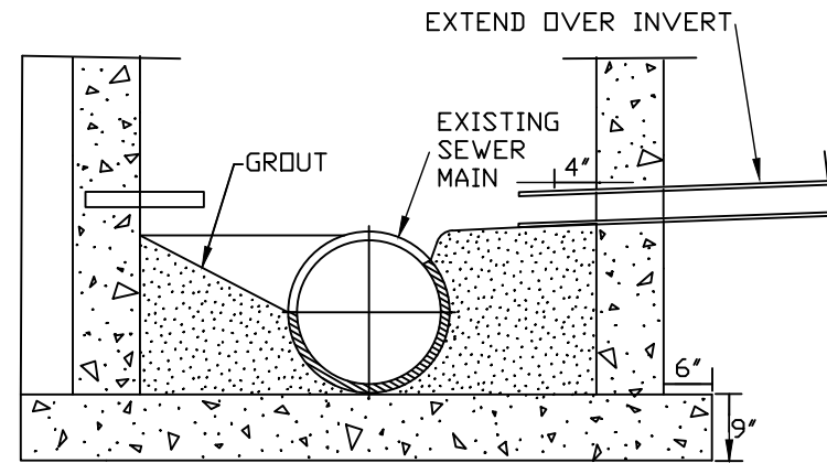
SECTION AT RIGHT ANGLE TO EXISTING MAIN
