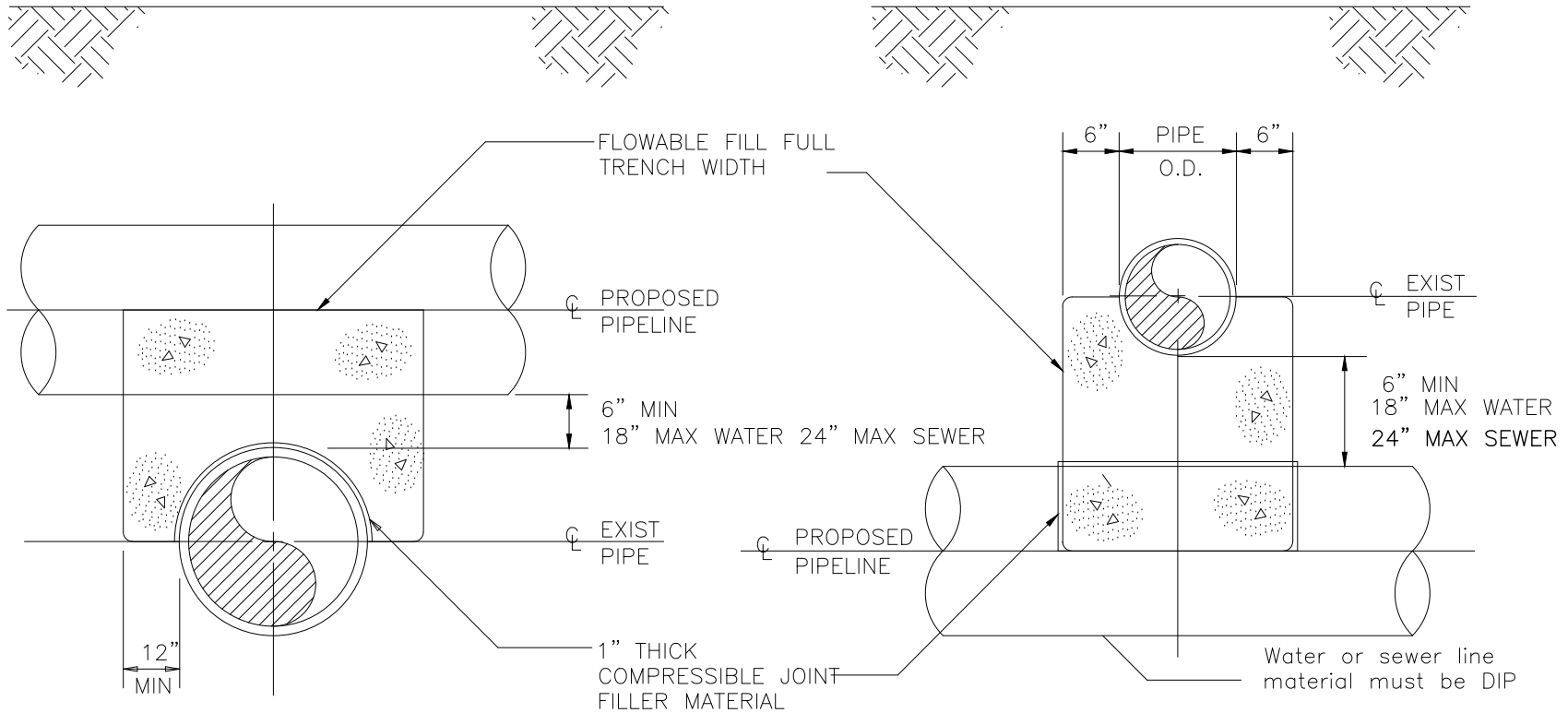
PROPOSED PIPELINE UNDER EXISTING PIPE
